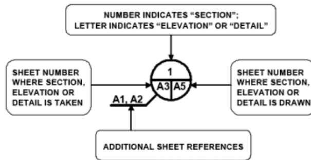
Figure 2-1. Standard Section Symbol
