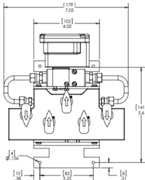
Figure 6-6. Transducer with 5-port Manifold
