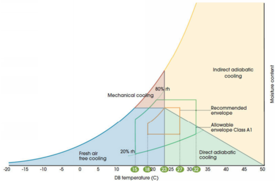
Diagram 1: Use of Ambient Air for Cooling as related to Humidity
