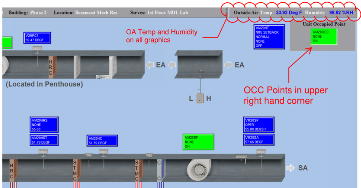
Figure 6-3. System Mode Points
