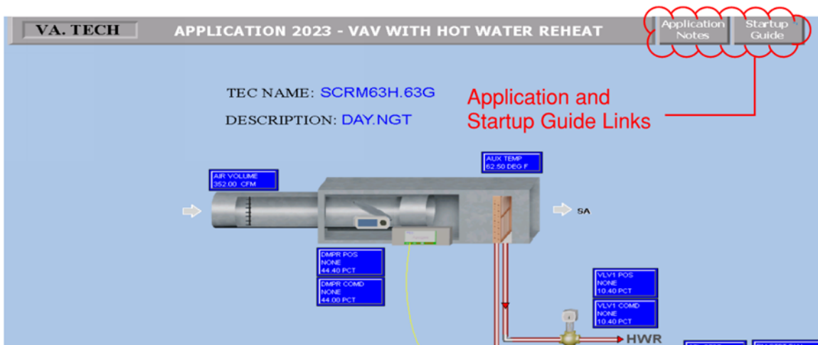
Figure 6-4. VAV Application Notes and Startup Guide
