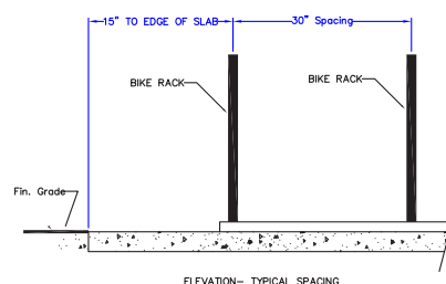
BIKE RACK DETAIL/ LAYOUT NOT TO SCALE
